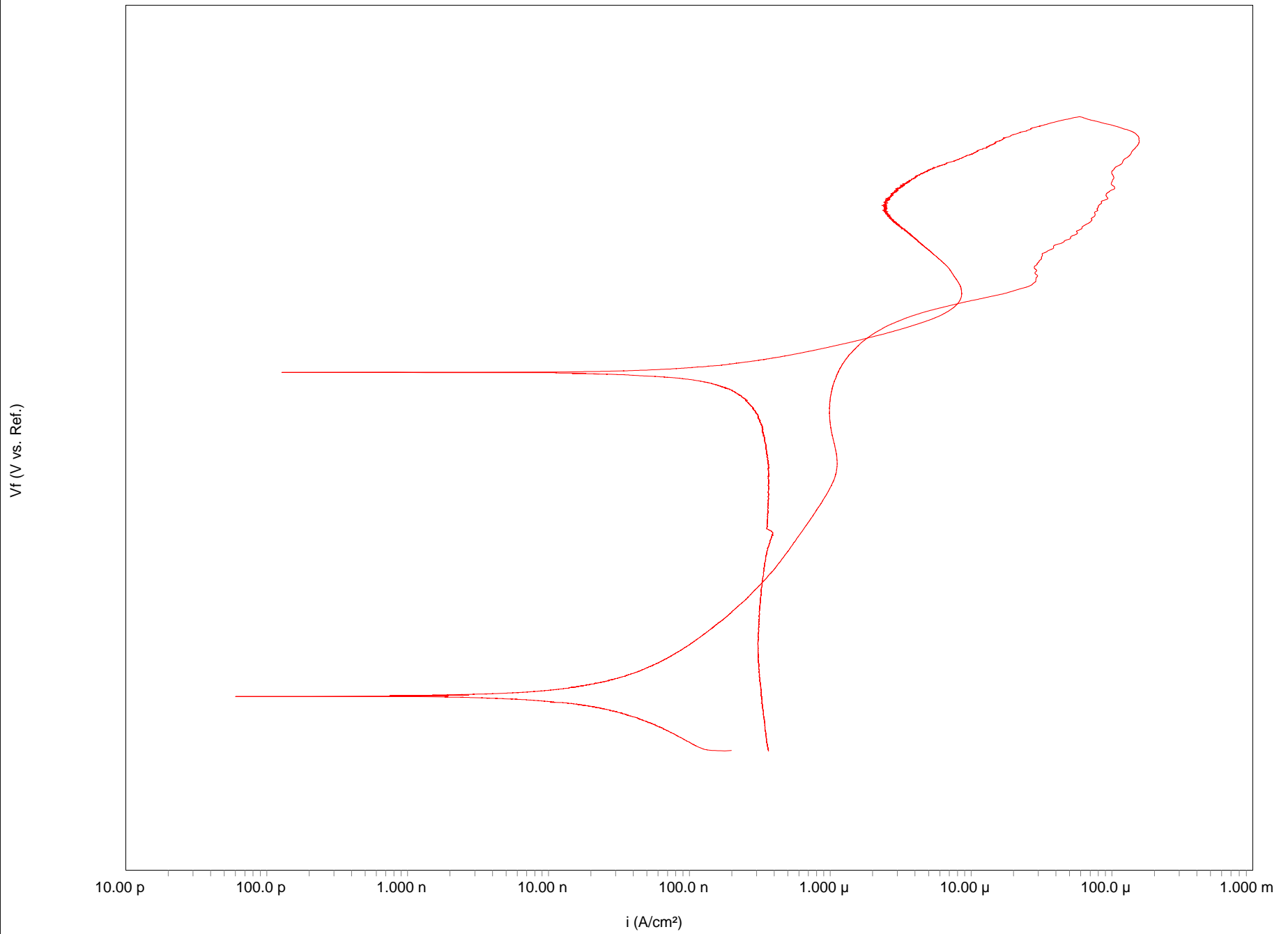
Sample Cyclic Polarization Scan
